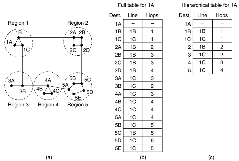
Figure 5-14. Hierarchical routing.
